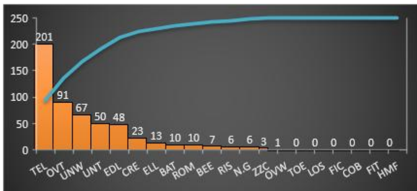
Figure 3 Pareto chart of number of defective Coils for March
